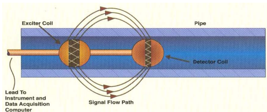
• Figure 1. Schematic of magnetic interaction between RFT tool and Pipe
